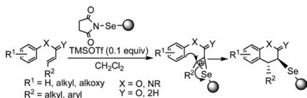
Scheme 1. Selenium-Promoted Intramolecular F–C Alkylation with Tethered Alkenes
