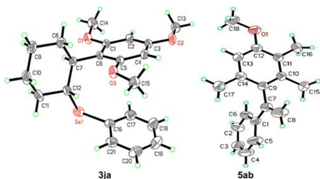
Figure 1. ORTEP structures of compounds 3ja and 5ab .
