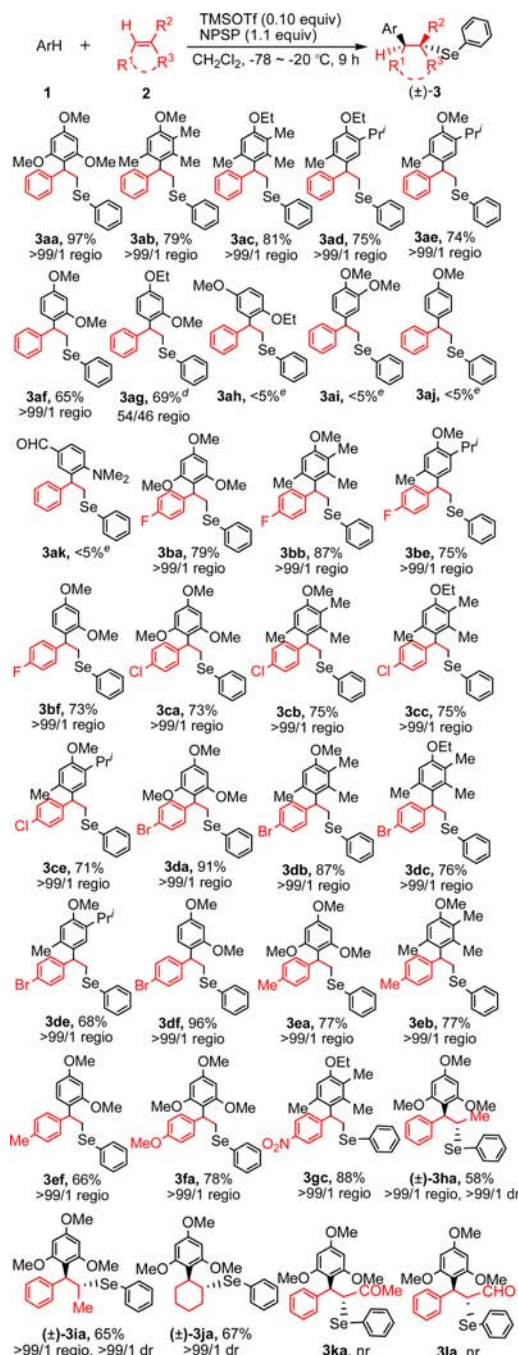
Scheme 2. Scope of Intermolecular Selenium-Promoted F–C Alkylation with Alkenes a–c
