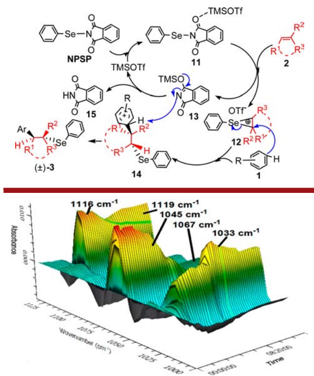
Figure 2. ReactIR spectrum of the F–C alkylation reaction of compound 1b with styrene and NPSP: 1-methoxy-2,3,5-trimethylbenzene ( 1b ), ( \nu C–O–C) 1116 \text{cm}^{-1} ; 15 , 1067 \text{cm}^{-1} ; 3ab , ( \nu C–O–C) 1119 \text{cm}^{-1} ; NPSP, 1045 \text{cm}^{-1} ; 13 , ( \nu Si–O) 1033 \text{cm}^{-1} .
